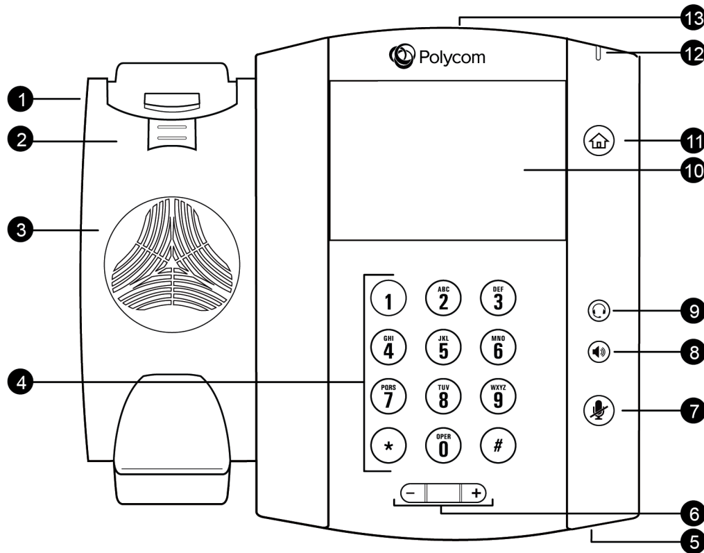
Figure 4: VVX 500 series and VVX 600 series hardware features
