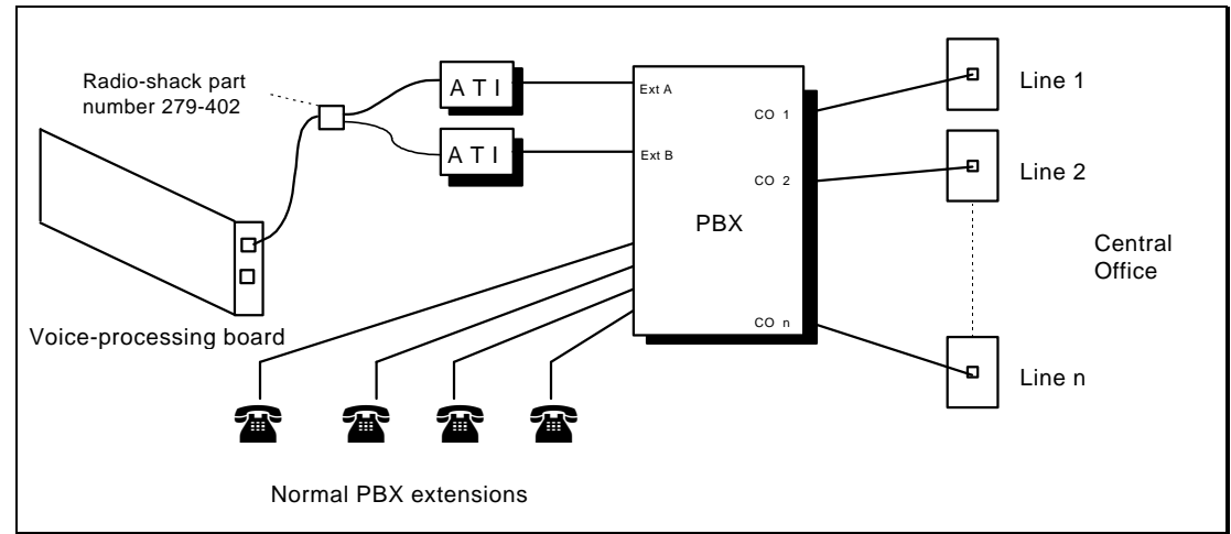
Connecting the Lite System to a PBX via External Analog Telephone Interface (ATI) Equipment
