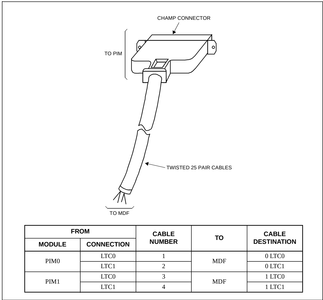
Figure 006-1 MDF Cable
