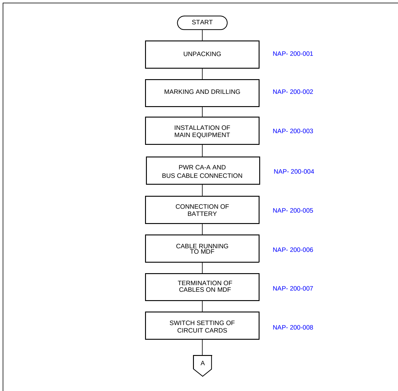
Figure 3-2 Procedure Flowchart
