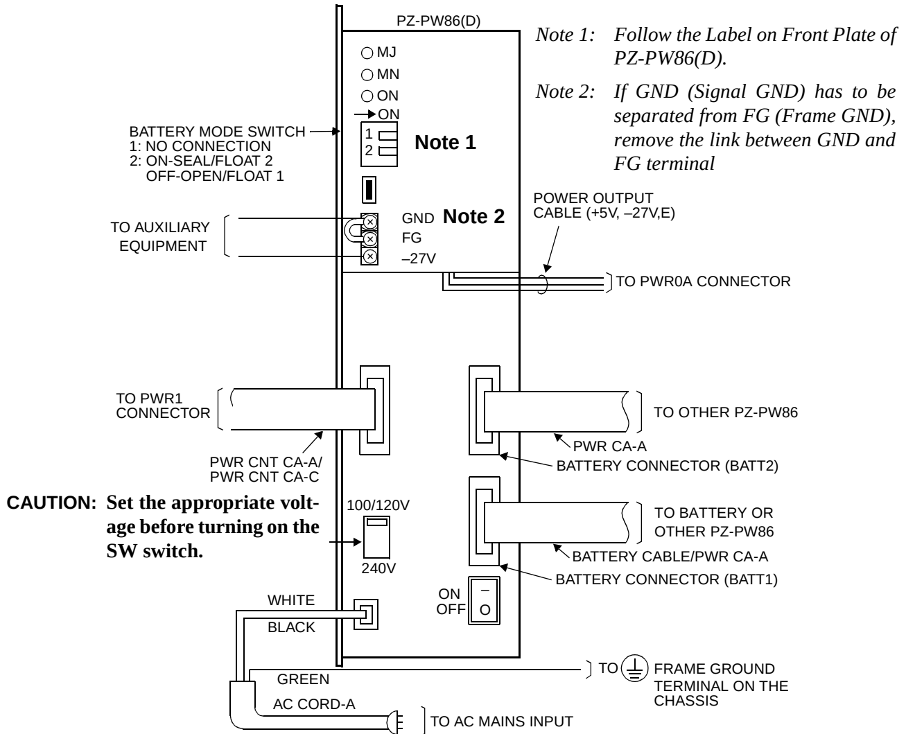
Figure 003-7 Cable Connection on PZ-PW86/PW112 (Continued)
