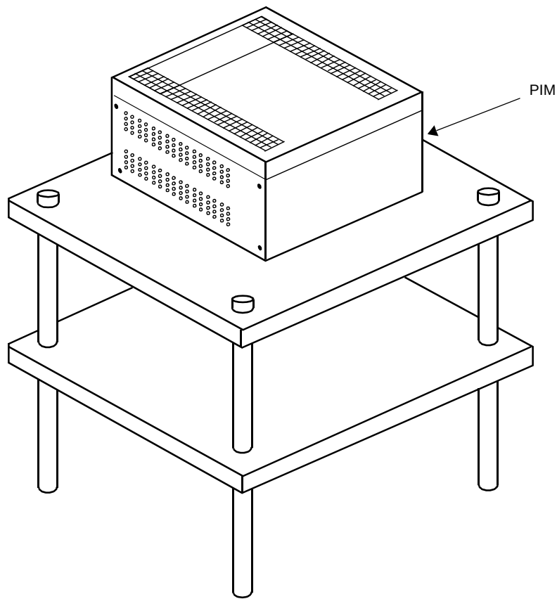
Figure 2-5 Desktop Installation
